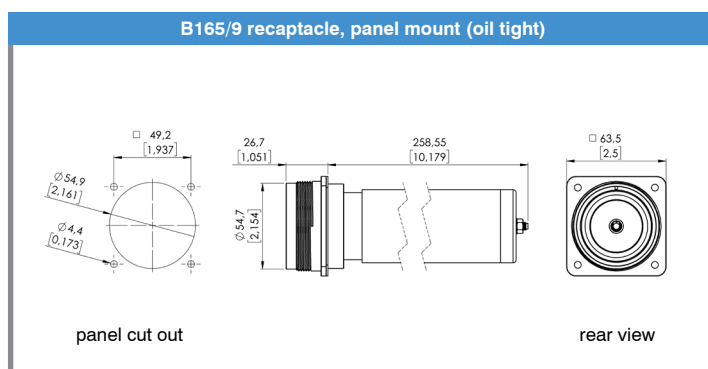
B 165/9 receptacle, panel mount
